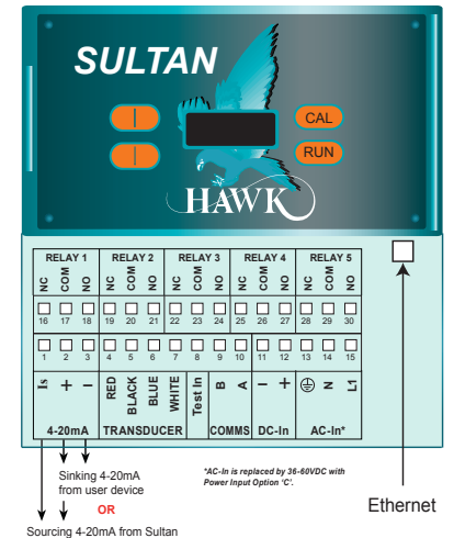
Unit with Internal Ethernet Connector
