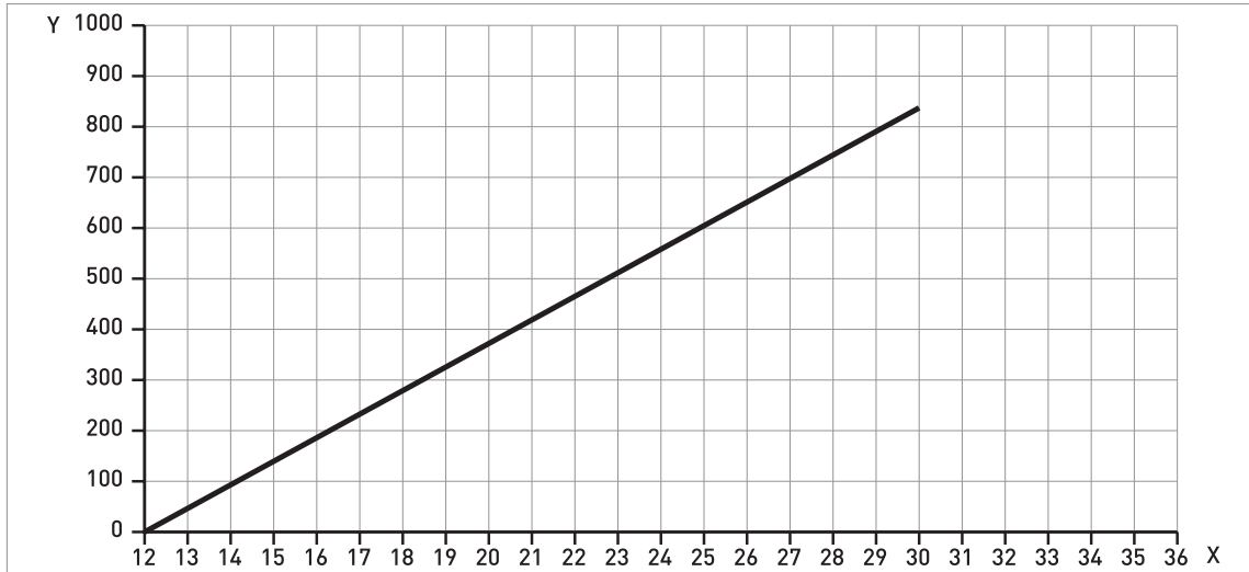
Figure 2-5: Minimum power supply voltage for an output of 21.5 mA at the terminals (Non-Ex and Hazardous Location approval (Ex i / IS))
